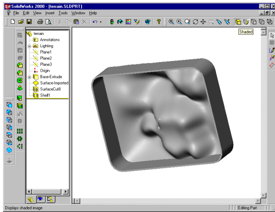
The new surface from below showing the shell feature intact.
